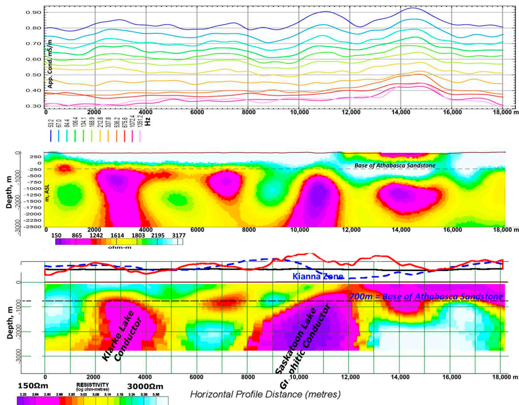
Figure 8. MobileMT apparent conductivity profiles (top); MobileMT resistivity section (middle) and ZTEM resistivity section (from [12], bottom) over the line crossing Kianna uranium mineralization zone.
