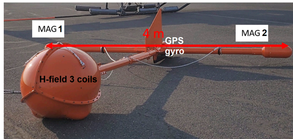
Figure 3. Airborne component of MobileMTm system.
